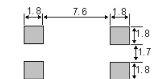
Recommended soldering pattern
