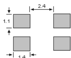
Recommended Soldering Pattern
