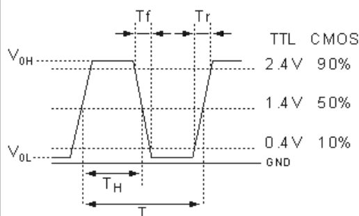
TTL / CMOS Output Wave Form
